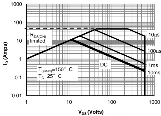
Figure 11: Maximum Forward Biased Safe Operating Area for AOD(I)380A60C (Note F)
