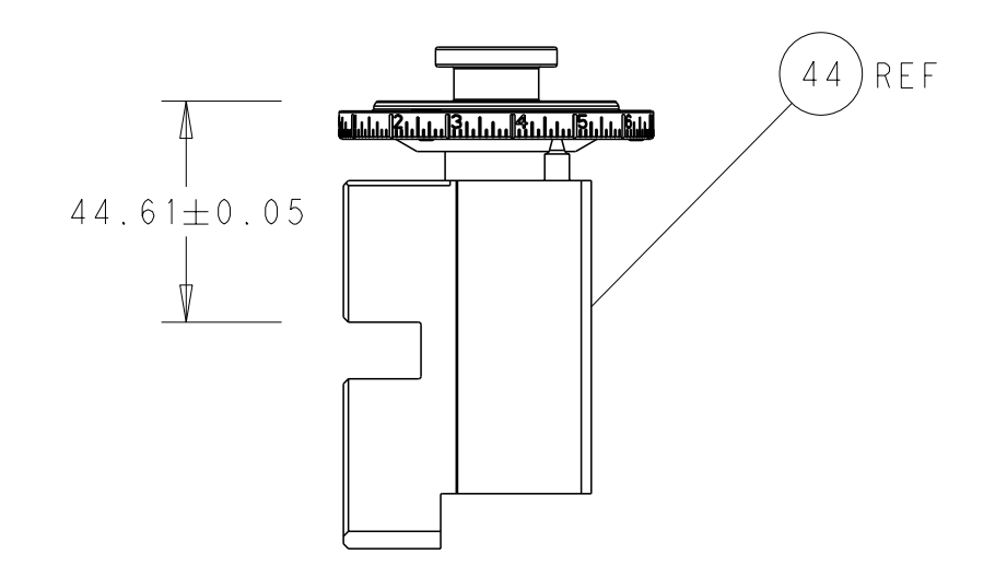
RAM SET-UP
