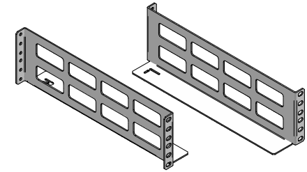
ISOMETRIC Sold with 2 Right and 2 Left
