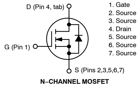
N-CHANNEL MOSFET
