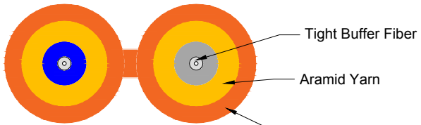
Cable Structure
