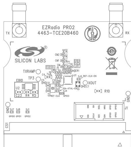
TOP ASSEMBLY TOP SILKSCREEN
