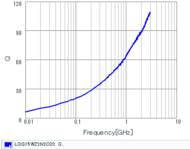
Q-Frequency Characteristics
