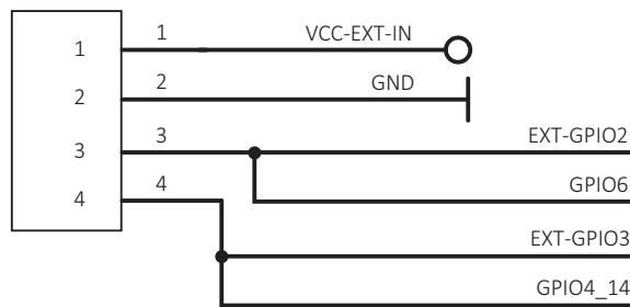
Figure 7: Adapter for Wandboard i.MX6 | I/O terminal, wiring diagram
