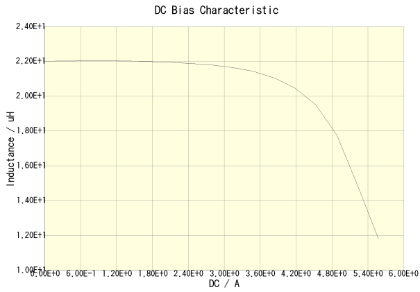
CLF12555T-220M-CA(Amb. Temp. = 20degc)
