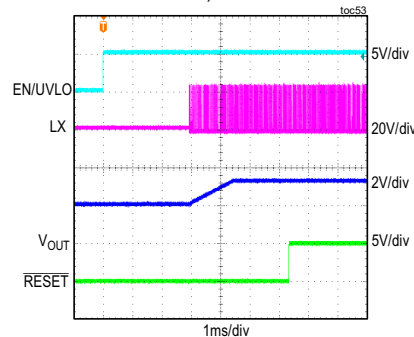
MAXM15064 STARTUP THROUGH ENABLE (2V PREBIAS) V_{IN} = 24V , ADJUSTABLE V_{OUT} = 3.3V , NO LOAD, PWM MODE
