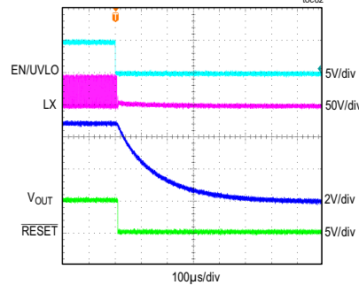
MAXM15063 SHUTDOWN THROUGH ENABLE V_{IN} = 48V , FIXED V_{OUT} = 5V , FULL LOAD, PWM MODE
