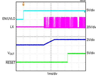
MAXM15062 STARTUP THROUGH ENABLE (2V PREBIAS) V_{IN} = 24V , FIXED V_{OUT} = 3.3V , NO LOAD, PWM MODE
