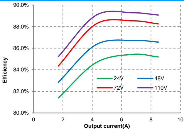
Figure 1: Efficiency vs. load current at 25°C.
