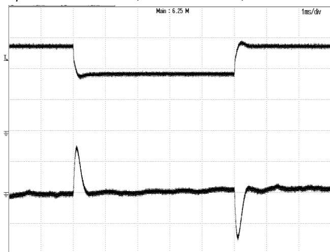
Figure 5: Output voltage response to step-change in load current (50%-75%-50% of full load; di/dt = 0.1A/\mu s ).
