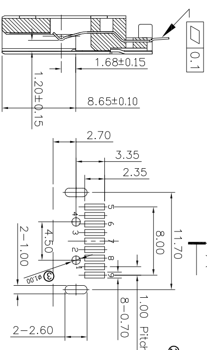
SECTION "A-A" RECOMMENDED P.C.B LAYOUT (TOLERANCE:±0.05)
