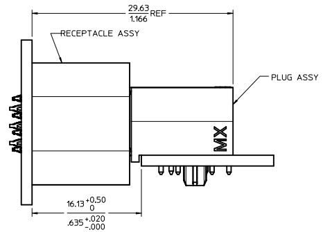
MATED PROFILE (SHOWN MATED TO VERTICAL RECEPTACLE ASSY)
