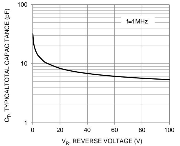
Figure 4. Typical Total Capacitance
