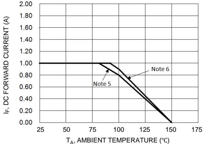
Figure 1. DC Forward Current Derating
