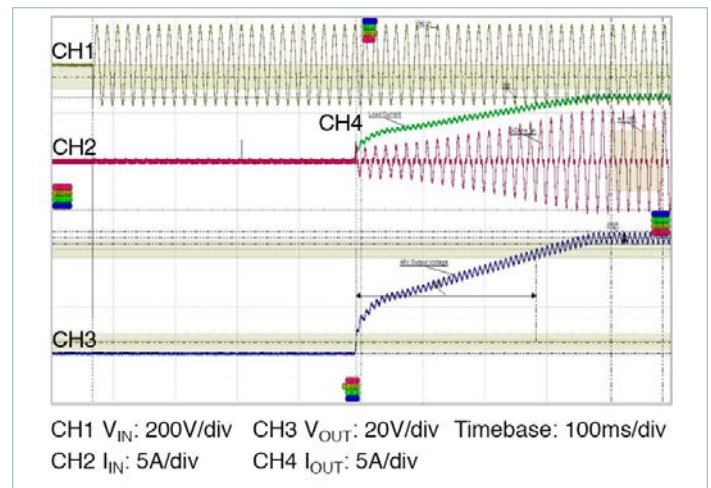
Figure 8 — Typical start-up waveform, application of V_{IN} , R_{LOAD} = 7.1\Omega , C_{OUT} = 6,800\mu F
