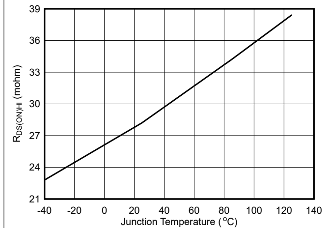
Figure 6-6. High-Side R_{DS(ON)}
