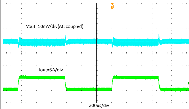
Figure 8-14. TPS565247 Transient Response with 0.1 A to 5 A by 2.5-A/ \mu s Load Step
