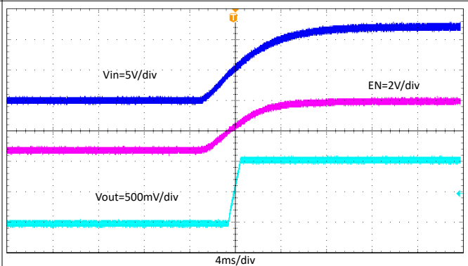
Figure 8-17. Start-Up with V_{IN} Rising, I_{OUT} = 5 A
