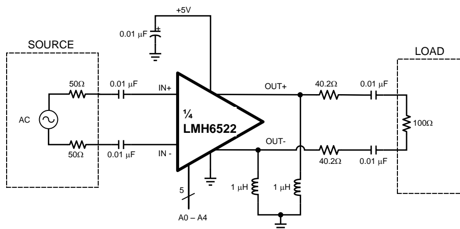
Figure 45. LMH6522 Basic Connections Schematic
