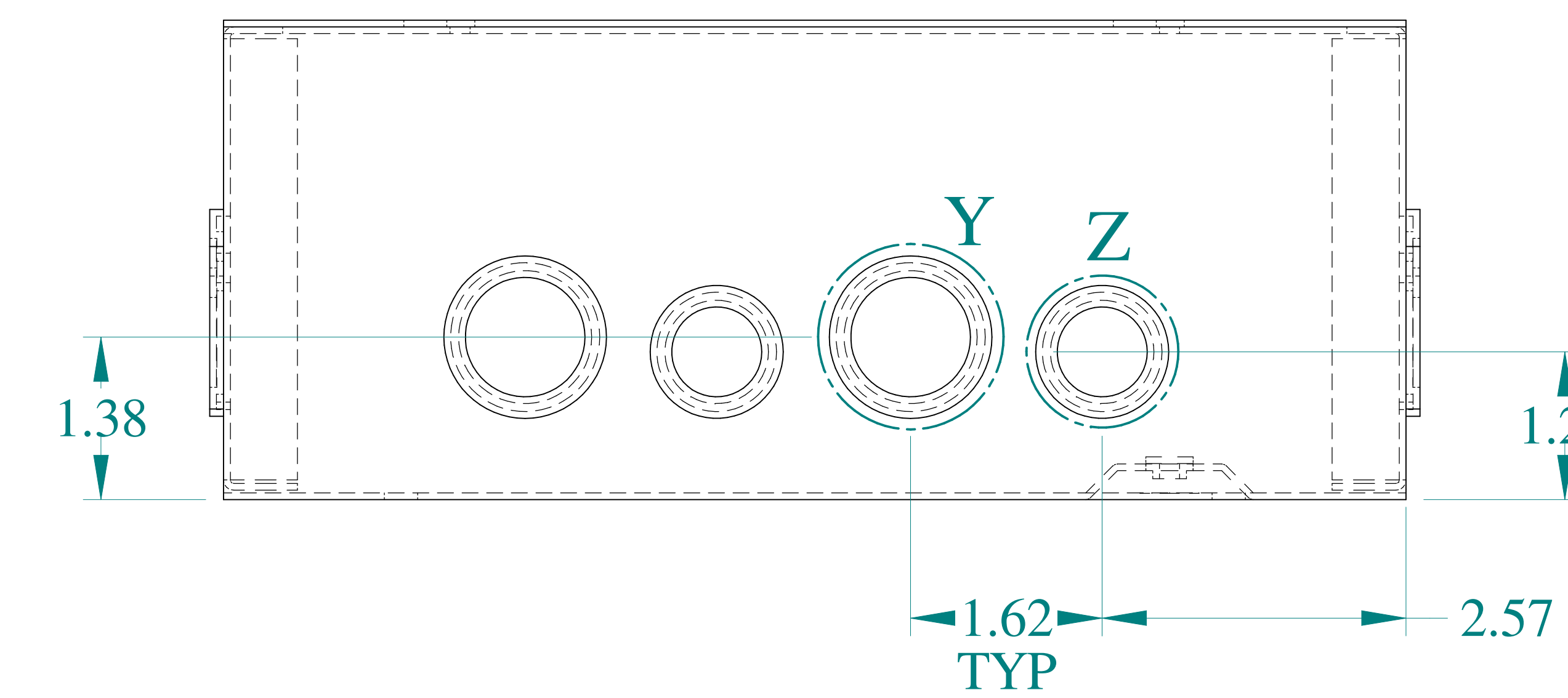
SIDE VIEW
