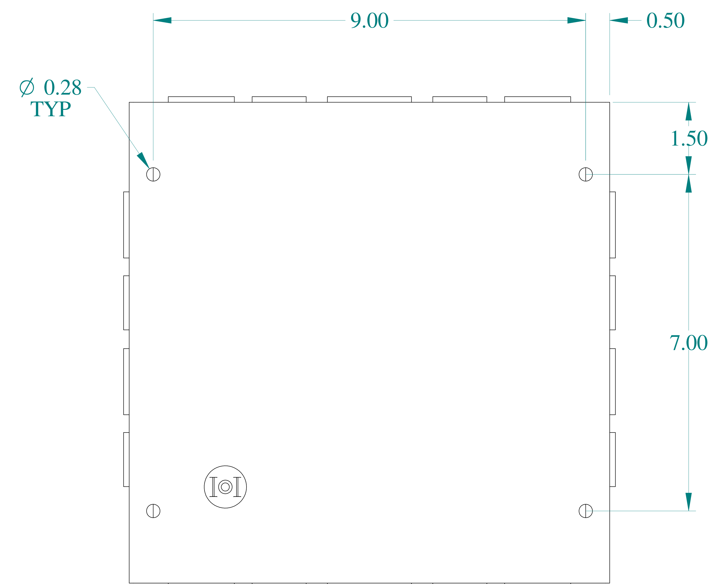
BOTTOM VIEW
