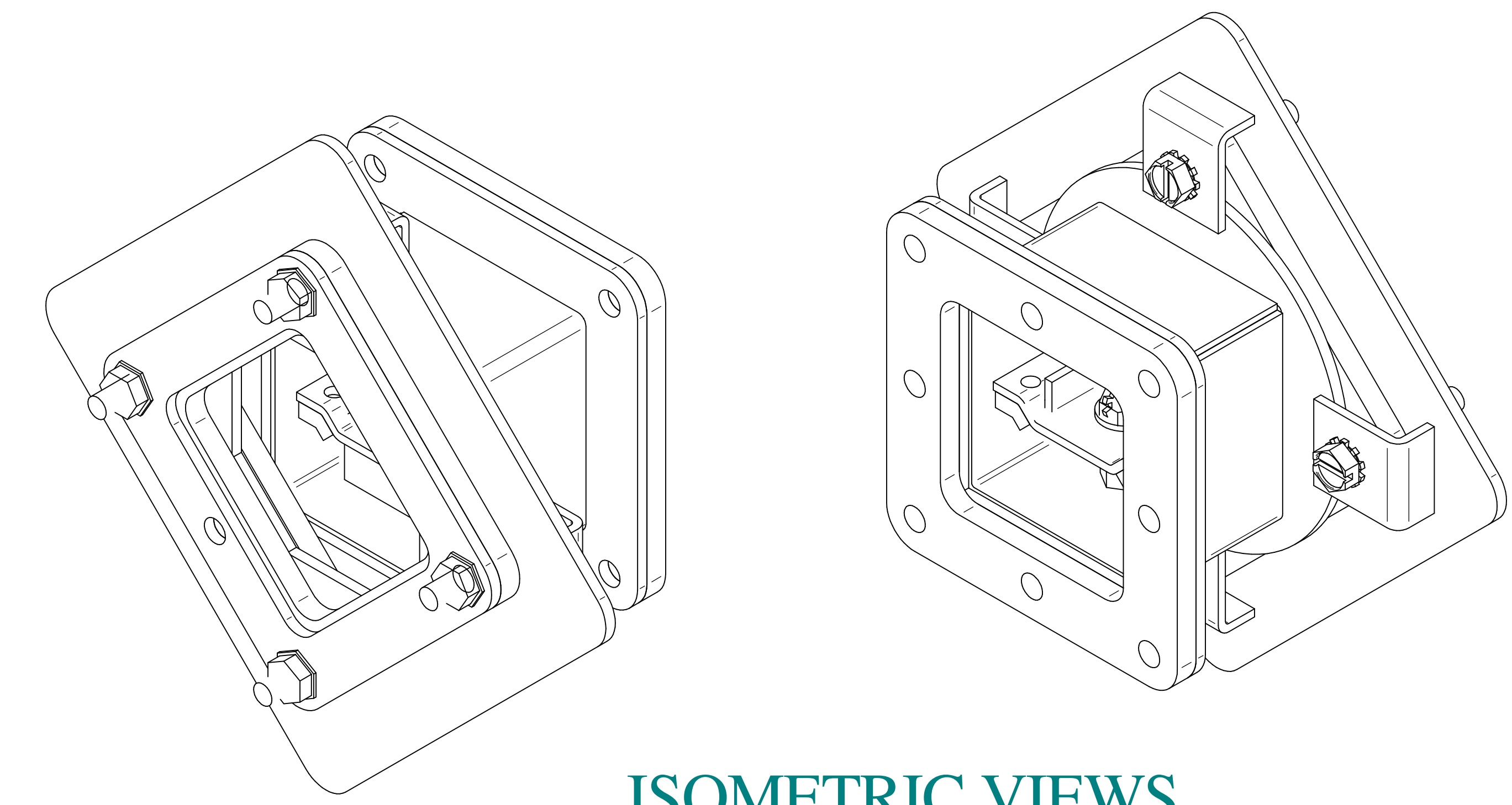
ISOMETRIC VIEWS
