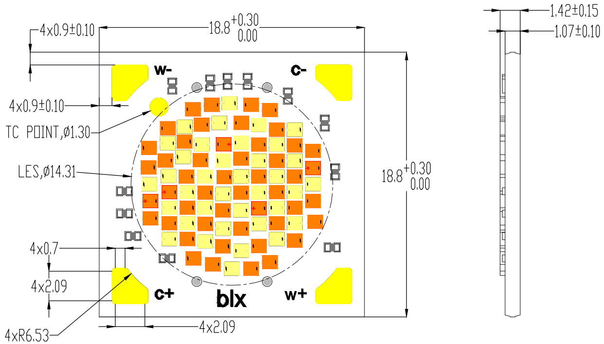
Figure 12: Drawing for Vesta Series Tunable White 13mm LED Array
