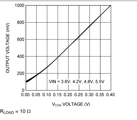
Figure 17. Low V_{CON} Voltage vs Output Voltage
