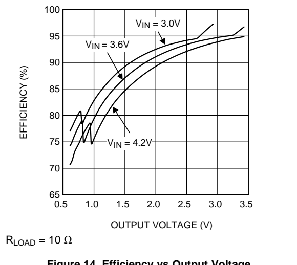
Figure 14. Efficiency vs Output Voltage
