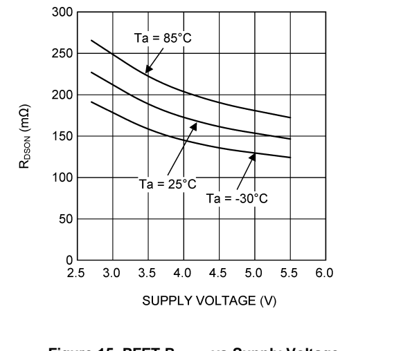
Figure 15. PFET R_{DS(on)} vs Supply Voltage
