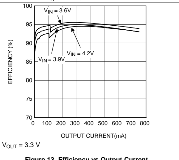
Figure 13. Efficiency vs Output Current
