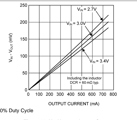
Figure 18. V_{IN} - V_{OUT} vs Output Current
