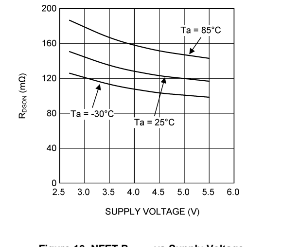
Figure 16. NFET R_{DS(on)} vs Supply Voltage
