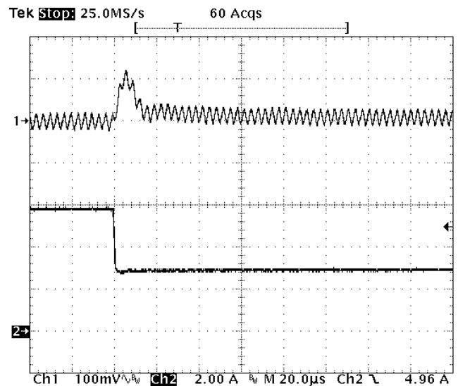
Fig-5.0V-7: Output voltage response for V_{out}=5.0V to negative load current step change from 6A to 3A with slew rate of -5A/\mu s at V_{in}=12V . C_o=47\mu F \times 2 ceramic.
