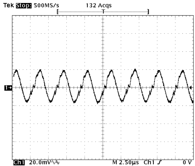
Fig-5.0V-5: Output voltage ripple (20mV/div.) for V_{out}=5.0V at full rated load current into a resistive load with external capacitance 47\mu F \times 2 ceramic + 1\mu F ceramic at V_{in}=12V .
