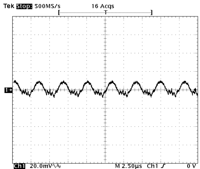
Fig-1.5V-5: Output voltage ripple (20mV/div.) for V_{out}=1.5V at full rated load current into a resistive load with external capacitance 47\mu F \times 2 ceramic + 1\mu F ceramic at V_{in}=12V .
