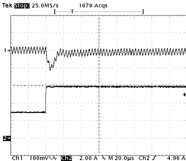
Fig-5.0V-6: Output voltage response for V_{out}=5.0V to positive load current step change from 3A to 6A with slew rate of 5A/\mu s at V_{in}=12V . C_o=47\mu F \times 2 ceramic.
