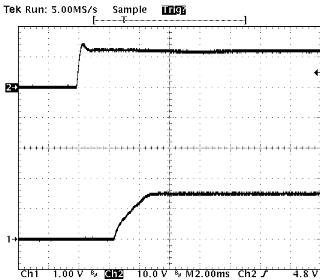
Fig-1.5V-4: Turn-on transient for V_{out}=1.5V with application of V_{in} at full rated load current (resistive) and 47\mu F \times 2 external capacitance at V_{in}=12V .
