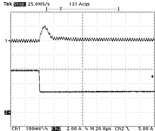
Fig-2.0V-7: Output voltage response for Vout=2.0V to negative load current step change from 6A to 3A with slew rate of -5A/us at Vin=12V. Co=47uFx2 ceramic. Top trace: output voltage (100mV/div.) Bottom trace: load current (2A/div.) Time scale: 20us/div.
