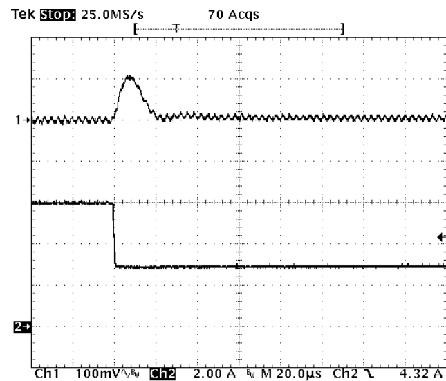
Fig-1.2V-7: Output voltage response for V_{out}=1.2V to negative load current step change from 6A to 3A with slew rate of -5A/\mu s at V_{in}=12V . C_o=47\mu F \times 2 ceramic. Top trace: output voltage (100mV/div.) Bottom trace: load current (2A/div.) Time scale: 20us/div.
