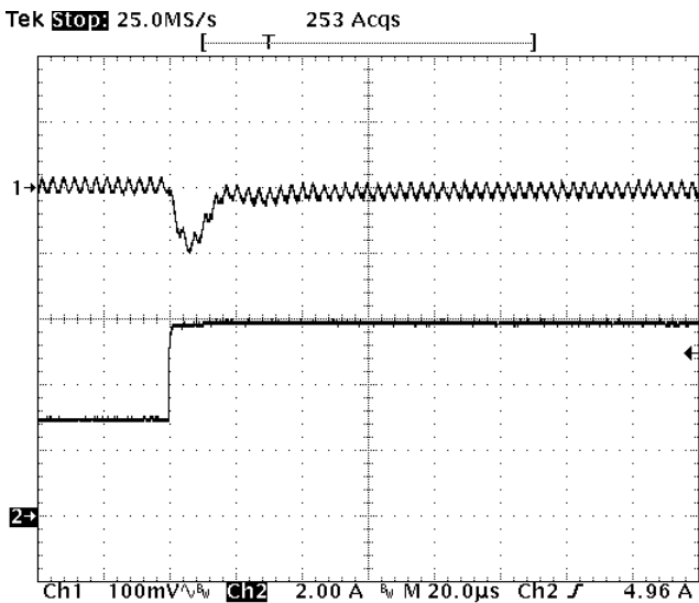
Fig-2.5V-6: Output voltage response for V_{out}=2.5V to positive load current step change from 3A to 6A with slew rate of 5A/\mu s at V_{in}=12V . C_o=47\mu F \times 2 ceramic. Top trace: output voltage (100mV/div.) Bottom trace: load current (2A/div.) Time scale: 20us/div.
