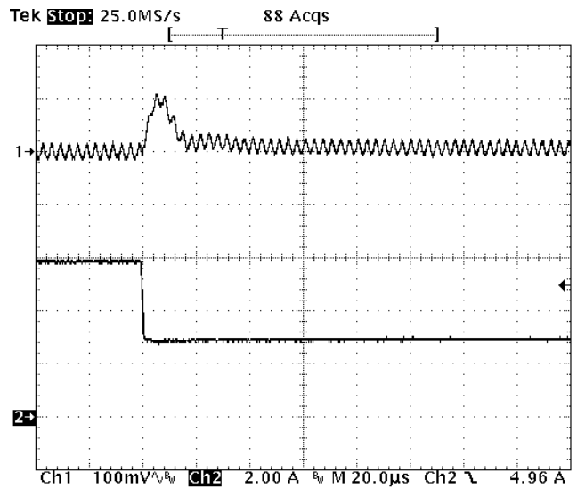
Fig-3.3V-7: Output voltage response for V_{out}=3.3V to negative load current step change from 6A to 3A with slew rate of -5A/\mu s at V_{in}=12V . C_o=47\mu F \times 2 ceramic. Top trace: output voltage (100mV/div.) Bottom trace: load current (2A/div.) Time scale: 20us/div.
