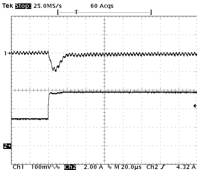
Fig-1.5V-6: Output voltage response for V_{out}=1.5V to positive load current step change from 3A to 6A with slew rate of 5A/\mu s at V_{in}=12V . C_o=47\mu F \times 2 ceramic.
