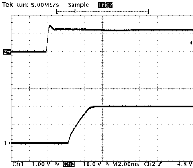
Fig-2.0V-4: Turn-on transient for Vout=2.0V with application of Vin at full rated load current (resistive) and 47uFx2 external capacitance at Vin=12V. Top trace: Vin (10V/div.) Bottom trace: output voltage (1V/div.) Time scale: 2 ms/div.
