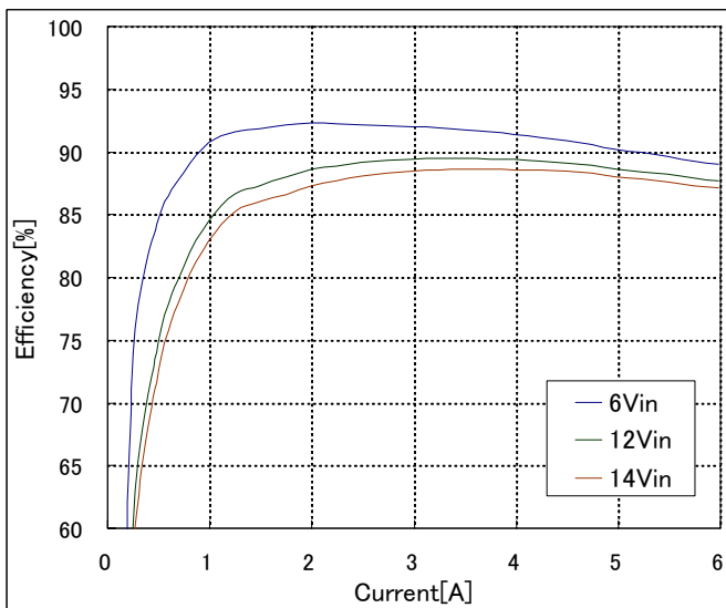
Fig-1.8V-2: Efficiency vs. load current and input voltage for V_{out}=1.8V . Airflow rate=200 LFM (1m/s) and T_a=25^{\circ}C .
