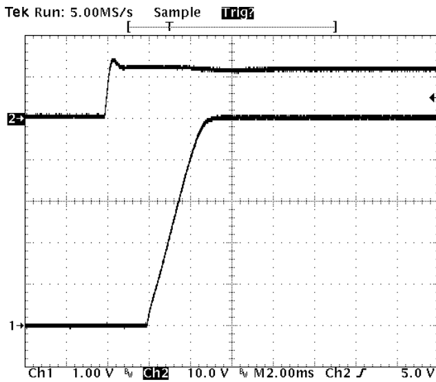
Fig-5.0V-4: Turn-on transient for V_{out}=5.0V with application of V_{in} at full rated load current (resistive) and 47\mu F \times 2 external capacitance at V_{in}=12V .
