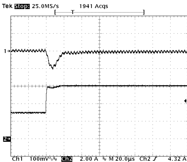
Fig-1.2V-6: Output voltage response for V_{out}=1.2V to positive load current step change from 3A to 6A with slew rate of 5A/\mu s at V_{in}=12V . C_o=47\mu F \times 2 ceramic. Top trace: output voltage (100mV/div.) Bottom trace: load current (2A/div.) Time scale: 20us/div.
