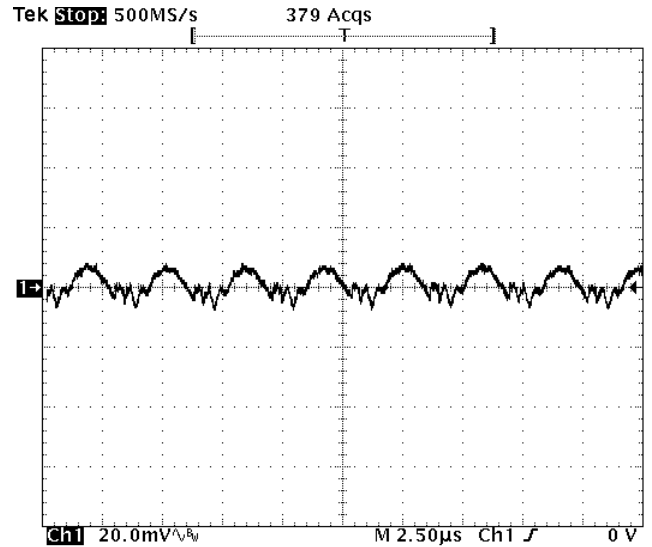
Fig-1.0V-5: Output voltage ripple (20mV/div.) for V_{out}=1.0V at full rated load current into a resistive load with external capacitance 47\mu F \times 2 ceramic + 1\mu F ceramic at V_{in}=12V . Time scale: 2.5 us/div
