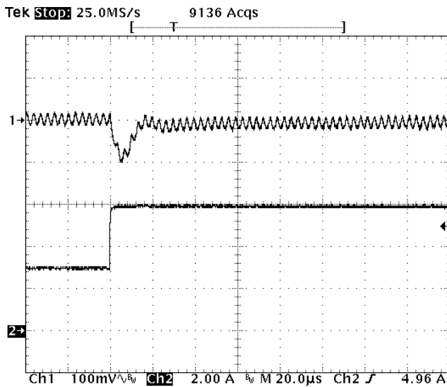
Fig-3.3V-6: Output voltage response for V_{out}=3.3V to positive load current step change from 3A to 6A with slew rate of 5A/\mu s at V_{in}=12V . C_o=47\mu F \times 2 ceramic. Top trace: output voltage (100mV/div.) Bottom trace: load current (2A/div.) Time scale: 20us/div.
