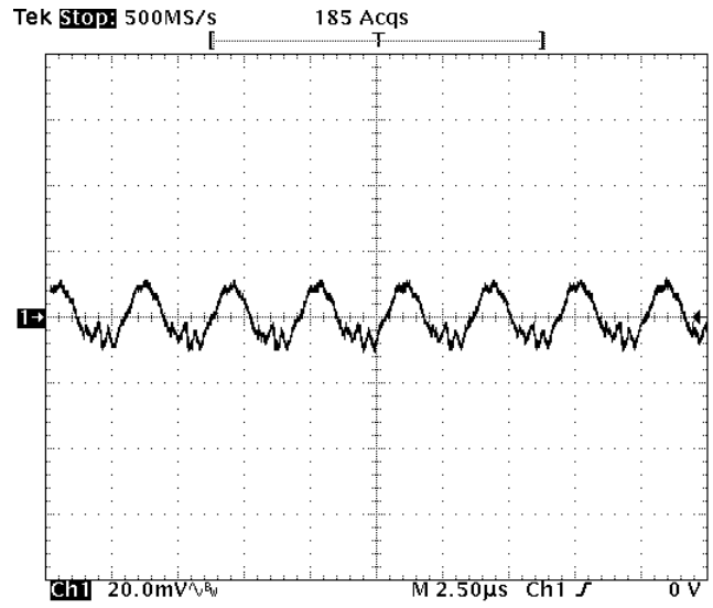
Fig-2.0V-5: Output voltage ripple (20mV/div.) for Vout=2.0V at full rated load current into a resistive load with external capacitance 47uFx2 ceramic + 1uF ceramic at Vin=12V. Time scale: 2.5 us/div.
