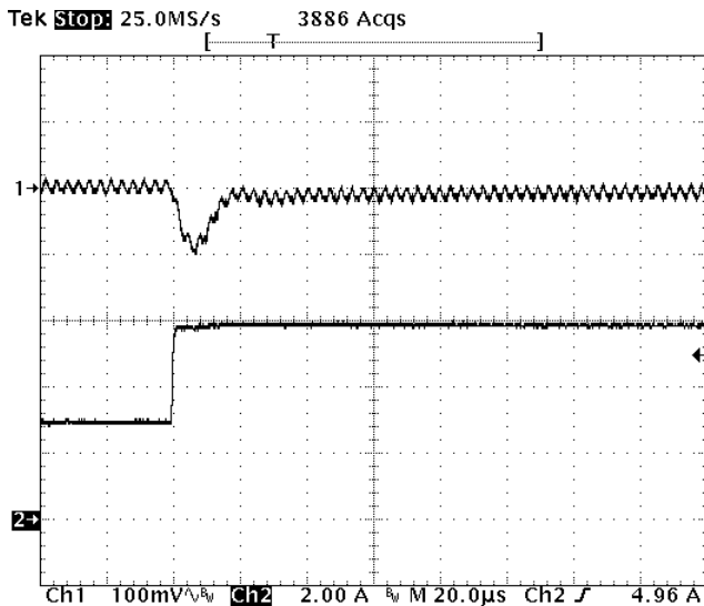
Fig-2.0V-6: Output voltage response for Vout=2.0V to positive load current step change from 3A to 6A with slew rate of 5A/us at Vin=12V. Co=47uFx2 ceramic. Top trace: output voltage (100mV/div.) Bottom trace: load current (2A/div.) Time scale: 20us/div.
