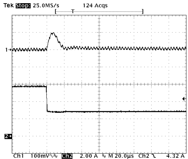
Fig-1.5V-7: Output voltage response for V_{out}=1.5V to negative load current step change from 6A to 3A with slew rate of -5A/\mu s at V_{in}=12V . C_o=47\mu F \times 2 ceramic.
