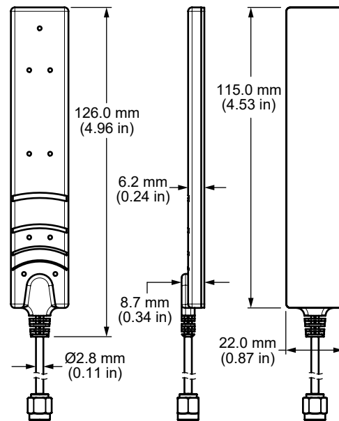
Figure 1. ANT-2/5-VDP-2000 Antenna Dimensions
