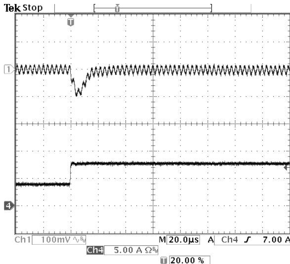
Fig-5.0V-6: Output voltage response for V_{out}=5.0V to positive load current step-change from 4A to 8A with slew rate of 5A/\mu s at V_{in}=12.0V . C_o=47\mu F \times 2 ceramic.
