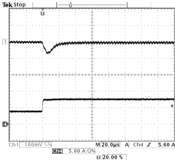
Fig-1.2V-6: Output voltage response for V_{out}=1.2V to positive load current step-change from 4A to 8A with slew rate of 5A/\mu s at V_{in}=12.0V . C_o=47\mu F \times 2 ceramic.
