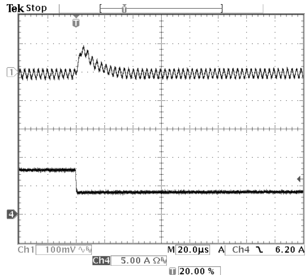
Fig-5.0V-7: Output voltage response for V_{out}=5.0V to negative load current step-change from 8A to 4A with slew rate of -5A/\mu s at V_{in}=12.0V . C_o=47\mu F \times 2 ceramic.
