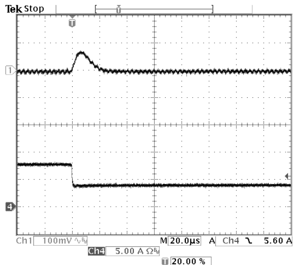
Fig-1.5V-7: Output voltage response for V_{out}=1.5V to negative load current step-change from 8A to 4A with slew rate of -5A/\mu s at V_{in}=12.0V . C_o=47\mu F \times 2 ceramic.
