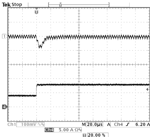
Fig-3.3V-6: Output voltage response for V_{out}=3.3V to positive load current step-change from 4A to 8A with slew rate of 5A/\mu s at V_{in}=12.0V . C_o=47\mu F \times 2 ceramic.
