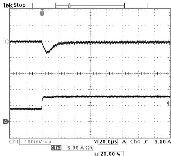
Fig-1.0V-6: Output voltage response for V_{out}=1.0V to positive load current step-change from 4A to 8A with slew rate of 5A/\mu s at V_{in}=12.0V . C_o=47\mu F \times 2 ceramic.
