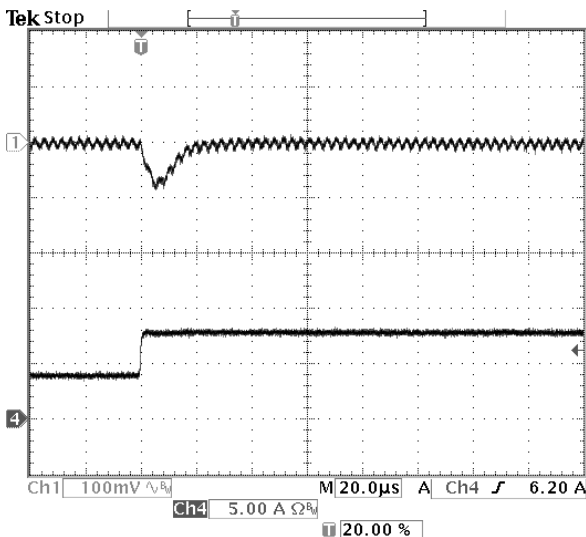
Fig-2.5V-6: Output voltage response for V_{out}=2.5V to positive load current step-change from 4A to 8A with slew rate of 5A/\mu s at V_{in}=12.0V . C_o=47\mu F \times 2 ceramic.
