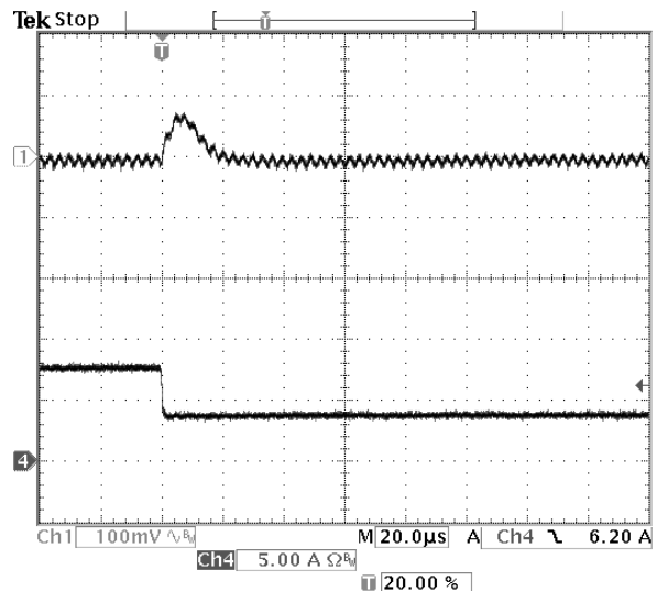
Fig-2.5V-7: Output voltage response for V_{out}=2.5V to negative load current step-change from 8A to 4A with slew rate of -5A/\mu s at V_{in}=12.0V . C_o=47\mu F \times 2 ceramic.
