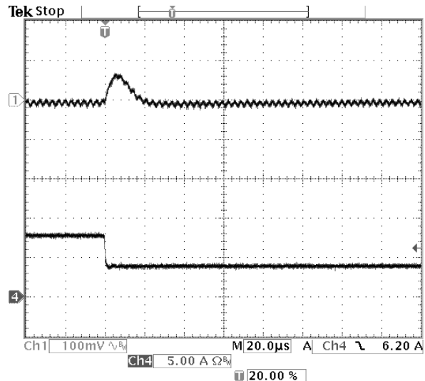
Fig-2.0V-7: Output voltage response for V_{out}=2.0V to negative load current step-change from 8A to 4A with slew rate of -5A/\mu s at V_{in}=12.0V . C_o=47\mu F \times 2 ceramic.
