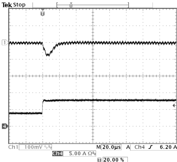
Fig-1.8V-6: Output voltage response for V_{out}=1.8V to positive load current step-change from 4A to 8A with slew rate of 5A/\mu s at V_{in}=12.0V . C_o=47\mu F \times 2 ceramic.
