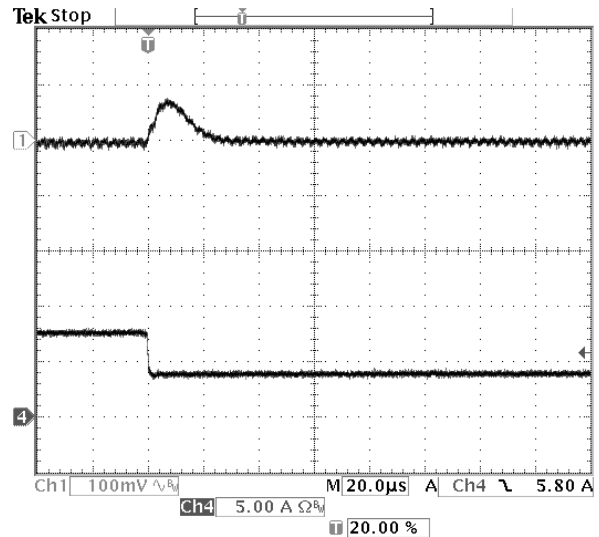
Fig-1.2V-7: Output voltage response for V_{out}=1.2V to negative load current step-change from 8A to 4A with slew rate of -5A/\mu s at V_{in}=12.0V . C_o=47\mu F \times 2 ceramic.
