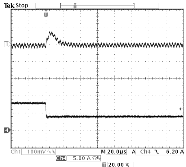
Fig-3.3V-7: Output voltage response for V_{out}=3.3V to negative load current step-change from 8A to 4A with slew rate of -5A/\mu s at V_{in}=12.0V . C_o=47\mu F \times 2 ceramic.
