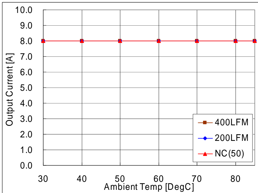
Fig-5.0V-1: Available load current vs. ambient temperature and airflow rates for Vout=5.0V with Vin=12.0V. Maximum component temperature \leq 120^{\circ}\text{C}
