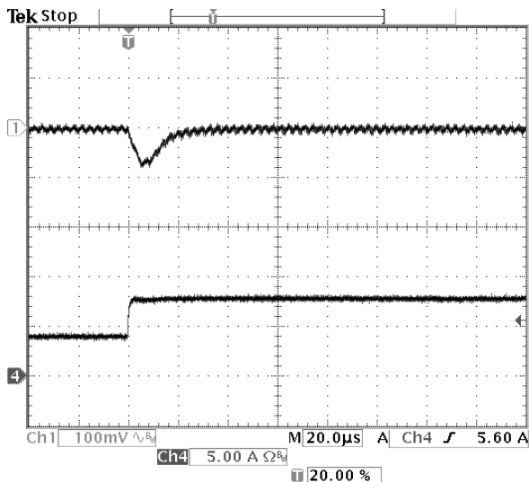
Fig-1.5V-6: Output voltage response for V_{out}=1.5V to positive load current step-change from 4A to 8A with slew rate of 5A/\mu s at V_{in}=12.0V . C_o=47\mu F \times 2 ceramic.
