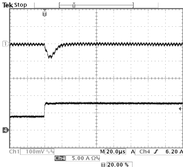
Fig-2.0V-6: Output voltage response for V_{out}=2.0V to positive load current step-change from 4A to 8A with slew rate of 5A/\mu s at V_{in}=12.0V . C_o=47\mu F \times 2 ceramic.
