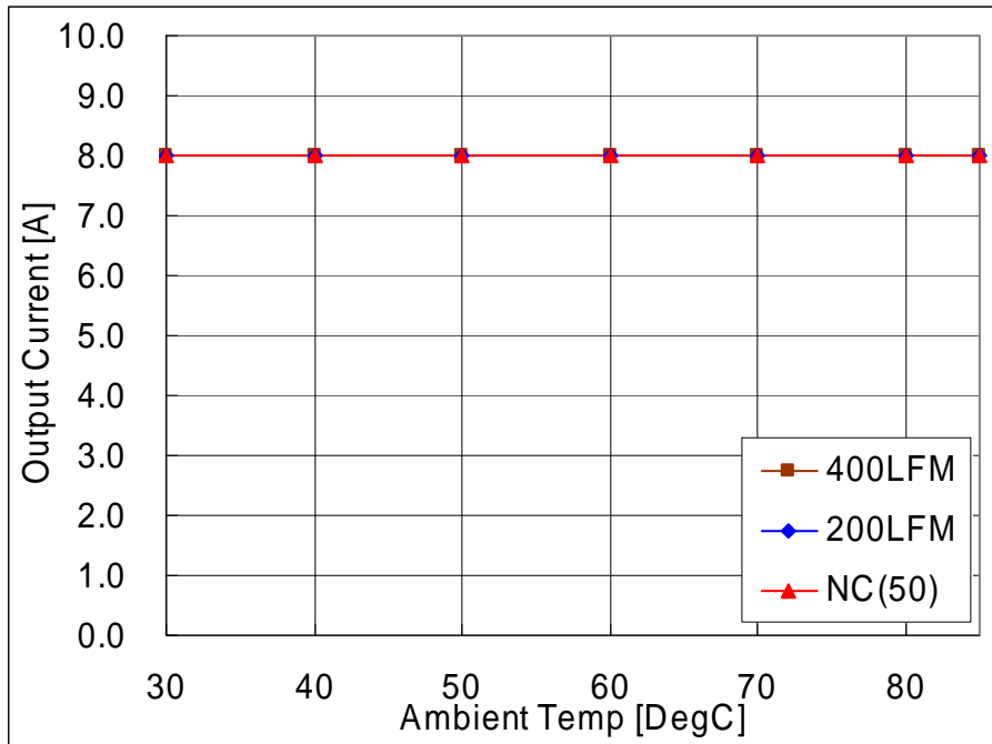
Fig-2.0V-1: Available load current vs. ambient temperature and airflow rates for Vout=2.0V with Vin=12.0V. Maximum component temperature ≤ 120°C
