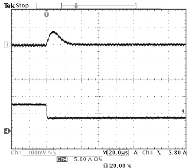
Fig-1.0V-7: Output voltage response for V_{out}=1.0V to negative load current step-change from 8A to 4A with slew rate of -5A/\mu s at V_{in}=12.0V . C_o=47\mu F \times 2 ceramic.
