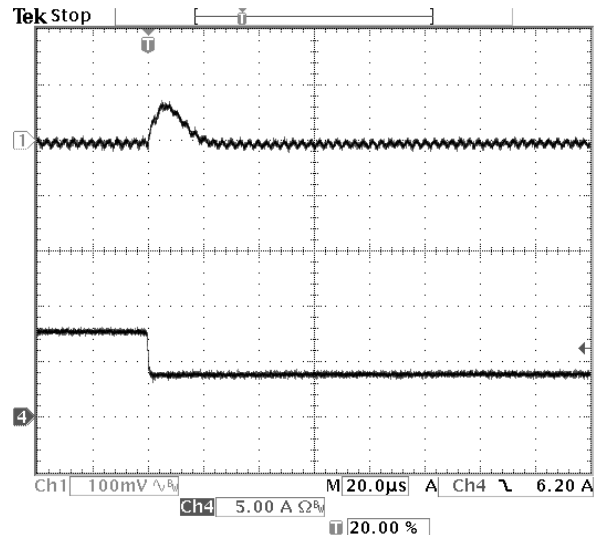
Fig-1.8V-7: Output voltage response for V_{out}=1.8V to negative load current step-change from 8A to 4A with slew rate of -5A/\mu s at V_{in}=12.0V . C_o=47\mu F \times 2 ceramic.
