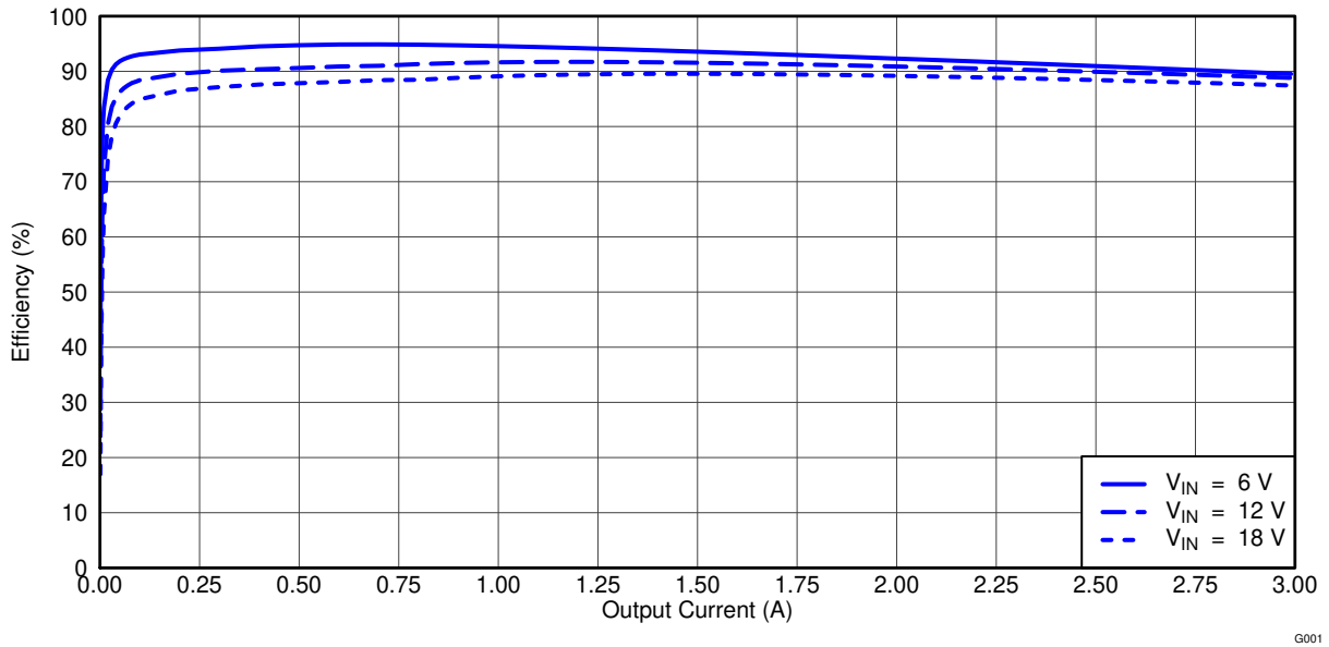
Figure 4-1. TPS54394EVM Converter 1 Efficiency
