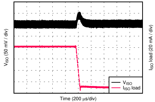
D042 Figure 8-11. V_{ISO} Load Transient Response, 90% to 10% Load Step, 5.0-V Input, 5.4-V Output
