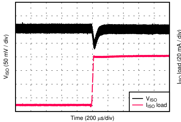
D041 Figure 8-10. V_{ISO} Load Transient Response, 10% to 90% Load Step, 5.0-V Input, 5.4-V Output
