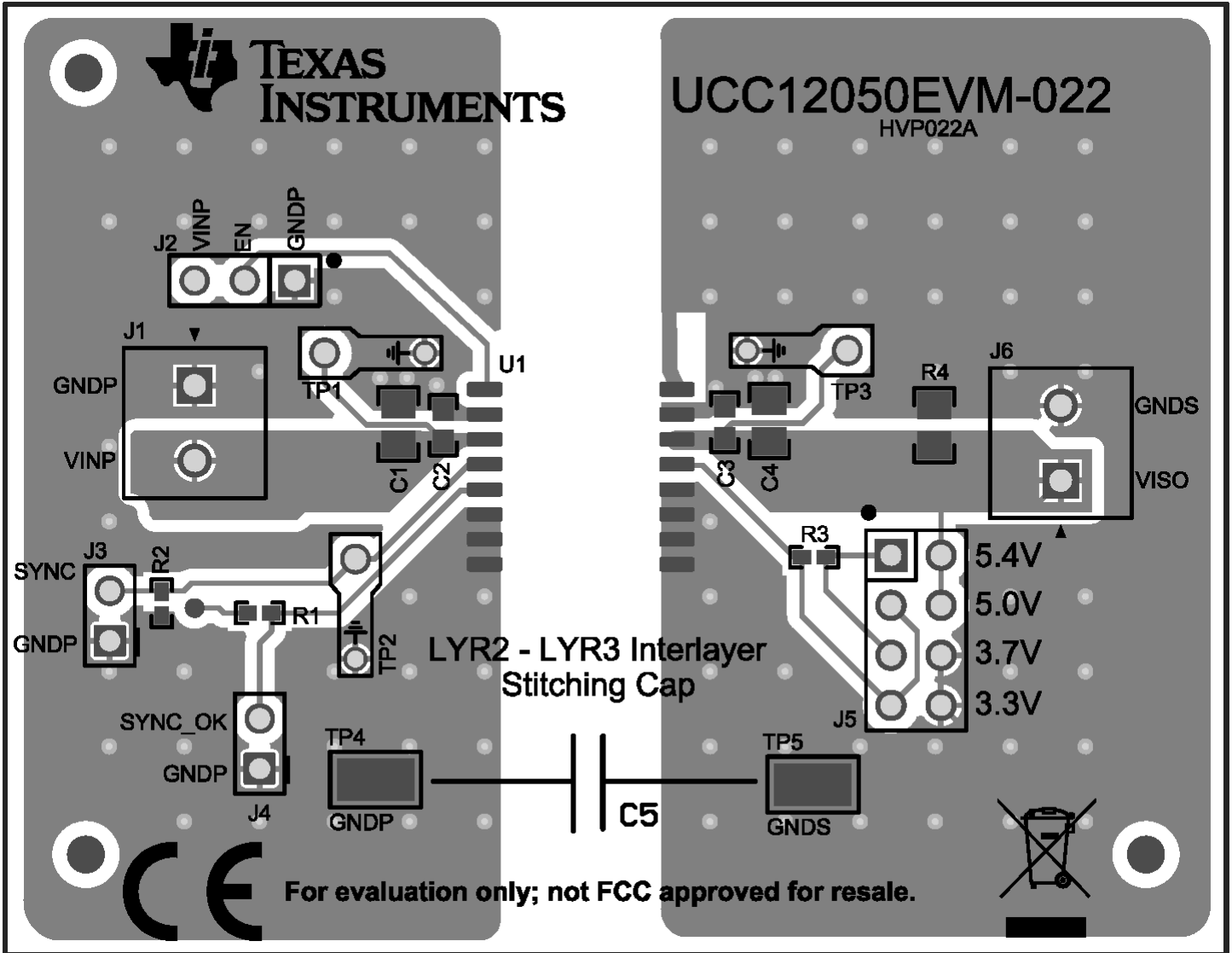
Figure 10-1. Layout Example
