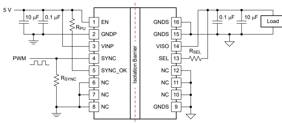
Figure 8-1. Typical Application
