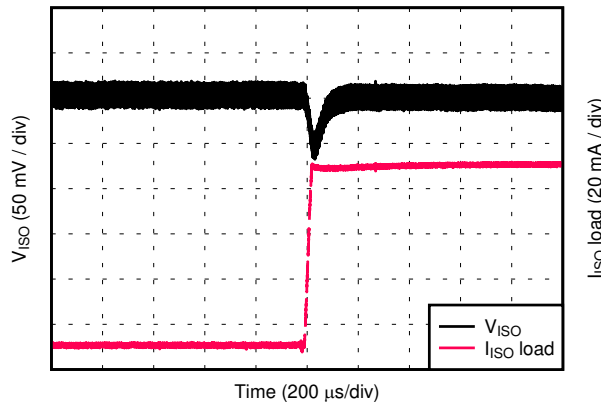
D043 Figure 8-12. V_{ISO} Load Transient Response, 10% to 90% Load Step, 5.0-V Input, 5.0-V Output
