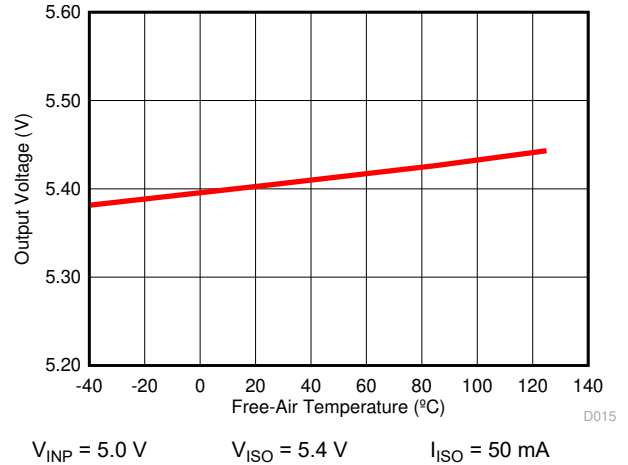
Figure 6-21. Isolated Supply Voltage ( V_{ISO} ) vs Free-Air Temperature
