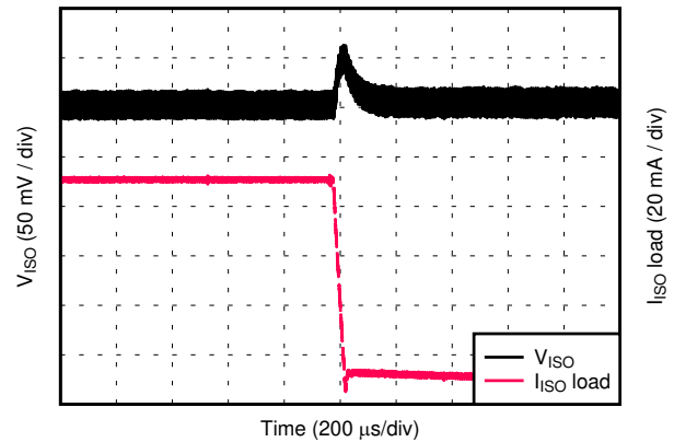
D044 Figure 8-13. V_{ISO} Load Transient Response, 90% to 10% Load Step, 5.0-V Input, 5.0-V Output
