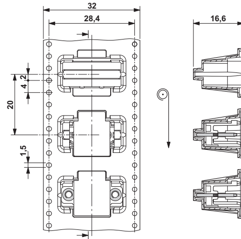
Dimensioned drawing
