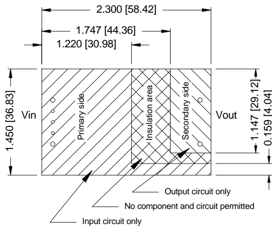
Figure 54. ORQB-50Y15L/0 Recommended pad layout-1
