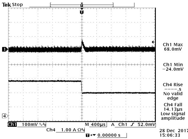
Figure 20. 75%-50% Load Transients at Vin=48V @Ta=25°C with Cext=200uF
