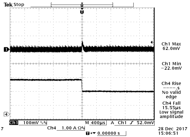
Figure 21. 75%-50% Load Transients at Vin=110V @Ta=25°C with Cext=200uF
