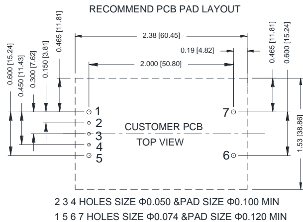
Figure 55. ORQB-50Y15L/0 Recommended pad layout-2
