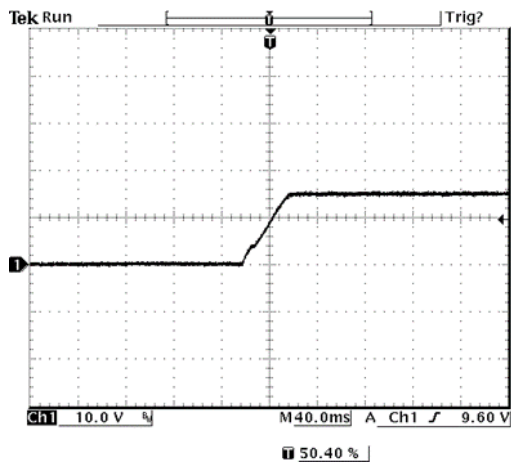
Figure 22. V_{in}=48V , I_o=3.3A , V_o=15V with C_{ext}=200\mu F
