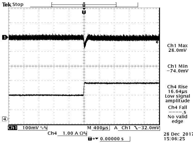
Figure 18. 50%-75% Load Transients at Vin=48V @Ta=25°C with Cext=200uF
