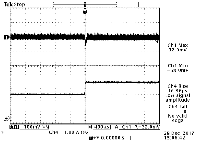
Figure 19. 50%-75% Load Transients at Vin=110V @Ta=25°C with Cext=200uF
