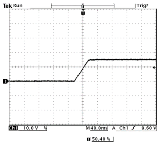
Figure 24. V_{in}=48V , I_o=3.3A , V_o=15V with C_{ext}=1200\mu F
