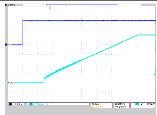
Figure 10-53. Start-Up Timing
