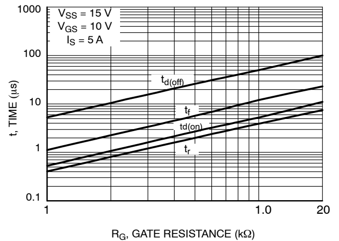
Figure 7. Switching Time vs. Gate Resistance
