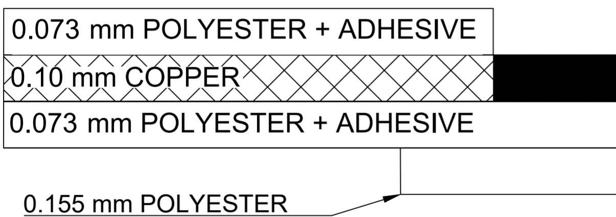
CROSS-SECTION
