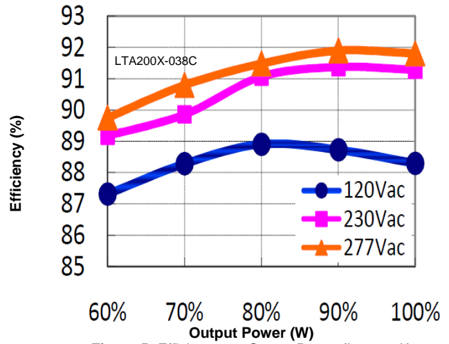
Figure 5: Efficiency vs. Output Power (Io=5.27A)
