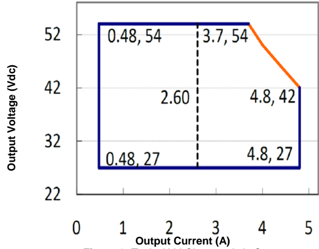
Figure 2: Typical V-I Characteristic Curve (LTA200X-054C)
