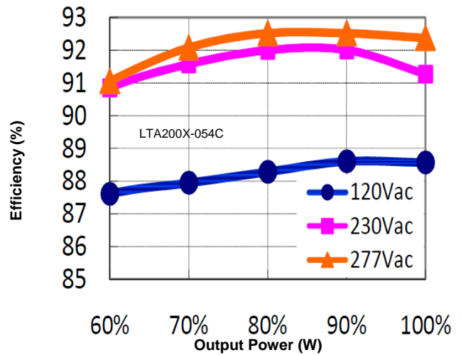
Figure 7: Efficiency vs. Output Power (Io=3.70A)
