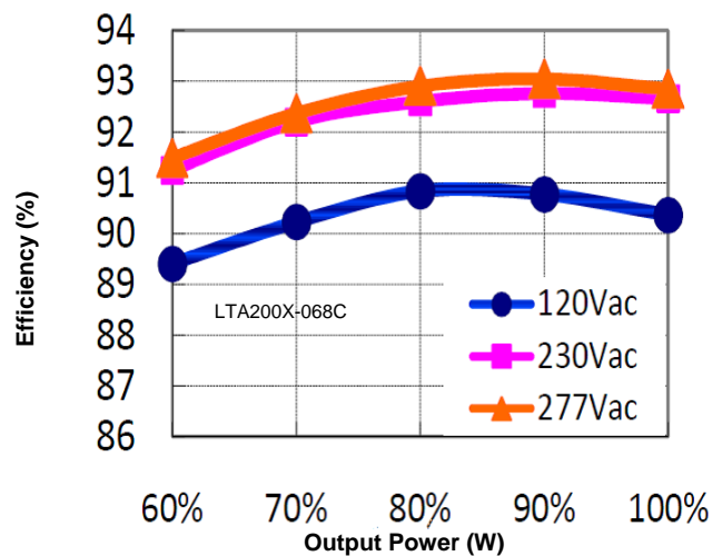
Figure 9: Efficiency vs. Output Power (Io=2.95A)
