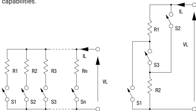
Figure 1. (left) Binary switching and (right) Optimized power switching
