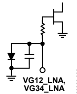
Figure 6. VG12_LNA and VG34_LNA Interface Schematic
