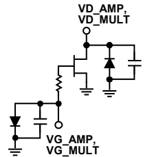
Figure 7. VG_MULT, VD_MULT, VG_AMP, and VD_AMP Interface Schematic
