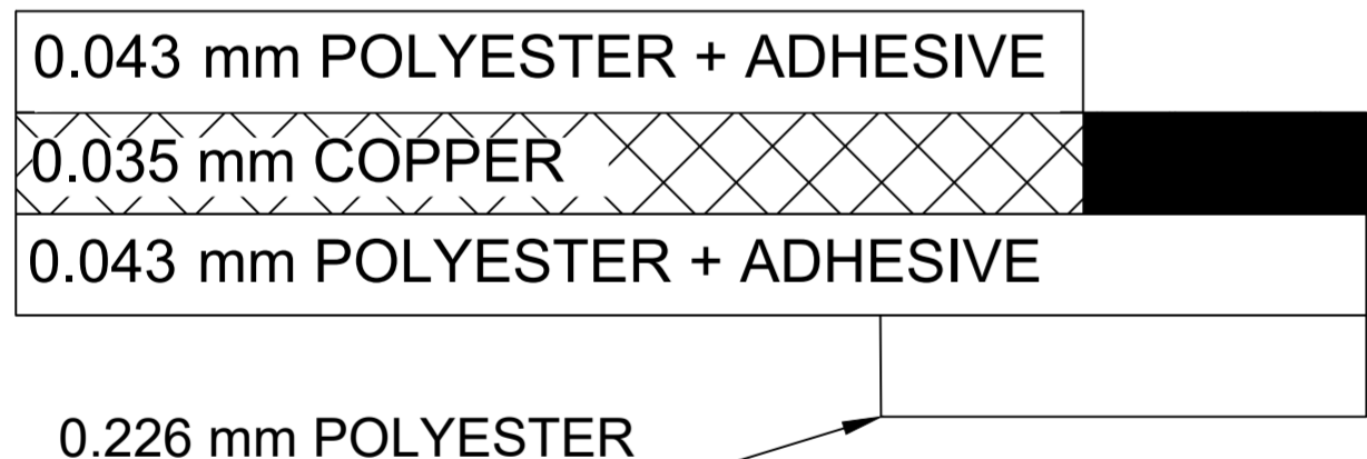
CROSS-SECTION
