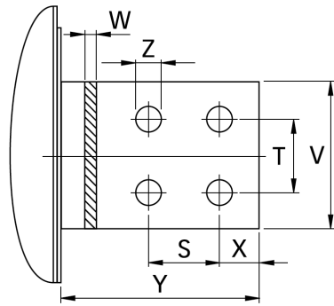
2500 A types
