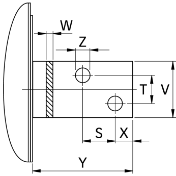
1600 A types
