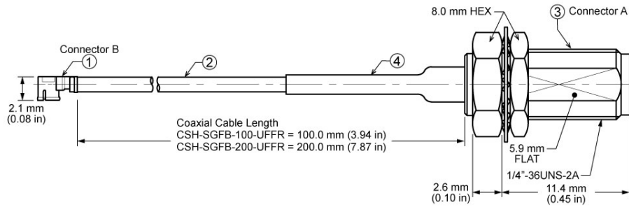
Figure 1. Product Dimensions for the CSH-SGFB-ccc-UFFR Cable Assembly
