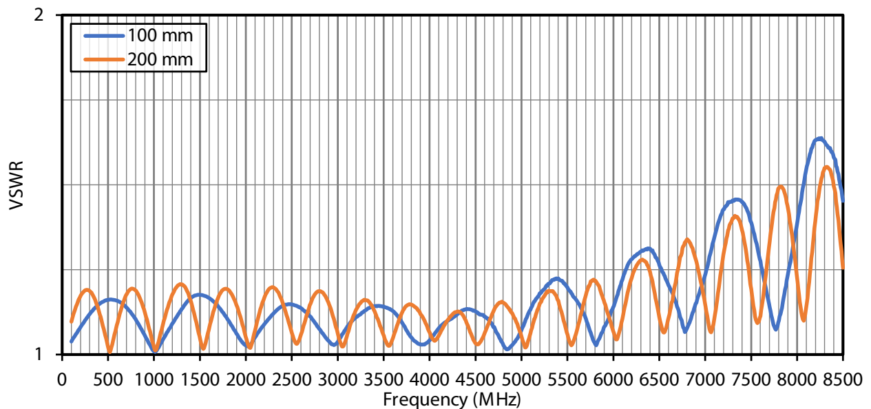
Figure 4. VSWR for the CSH-SGFB-ccc-UFFR Cable Assembly
