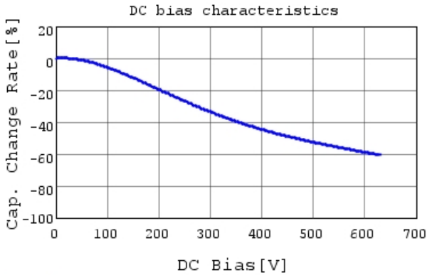
RDED72J473K3M1H03A C-DC bias capchange, 25.0
