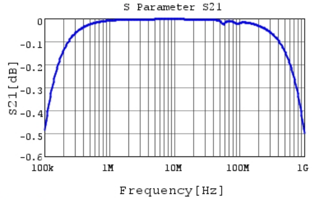
RDED72J473K3M1H03A S21 DCOV, 25degC
