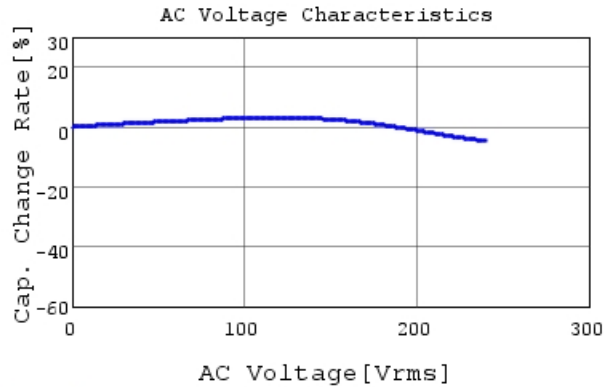
RDED72J473K3M1H03A C-AC Voltage capchange, I
