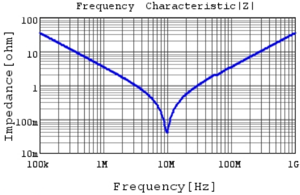
RDED72J473K3M1H03A |Z| DC0V,25degC
