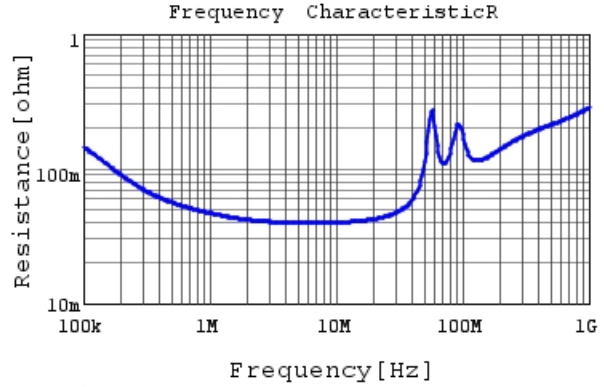
RDED72J473K3M1H03A R DC0V,25degC
