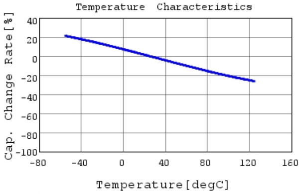
RDED72J473K3M1H03A C-Temp. capchange, DCOV,
