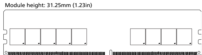
Figure 1: 288-Pin UDIMM (R/C D2)
