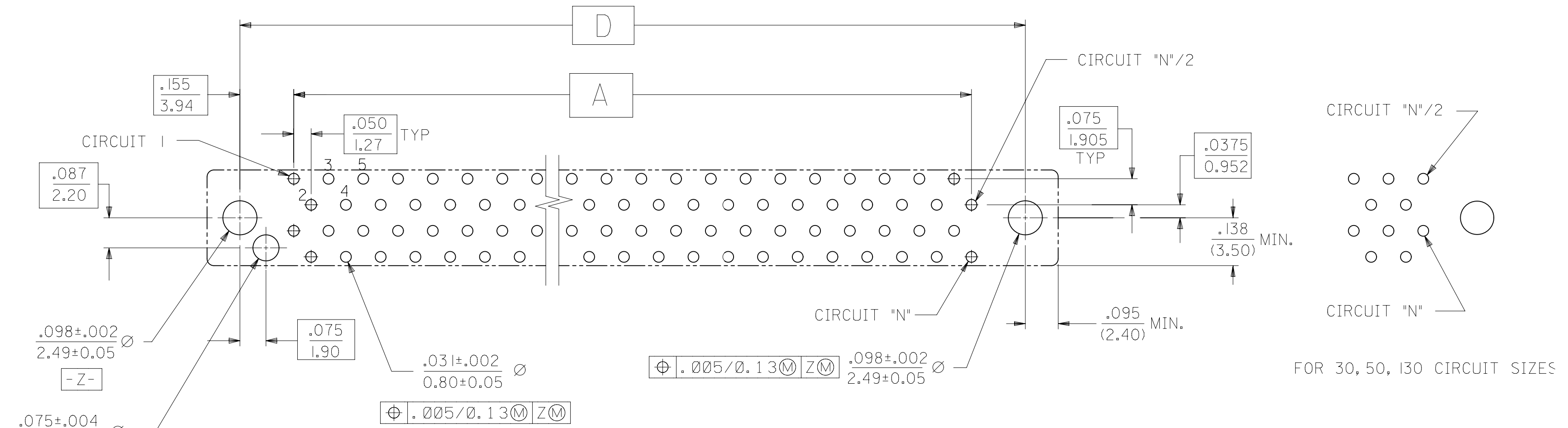
RECOMMENDED PC BOARD LAYOUT COMPONENT SIDE A FOR 40, 60, 68, 80, 100, 120 CIRCUIT SIZES
