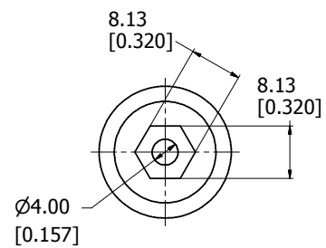
BACK FOOT
