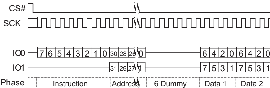
Figure 79. Dual I/O Read Command Sequence (4-Byte Address, BBh [ExtAdd=1], HPLC=10b)
