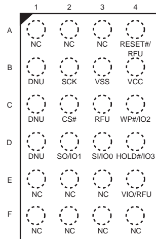
Figure 43. 24-Ball BGA, 4 x 6 Ball Footprint (FAC024), Top View
