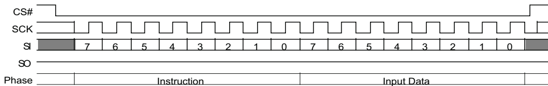
Figure 55. Bank Register Write (BRWR 17h) Command
