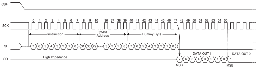
Figure 62. ECC Status Register Read Command Sequence
