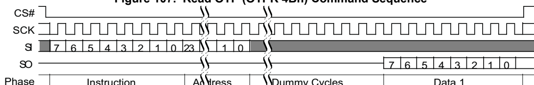
Figure 107. Read OTP (OTPR 4Bh) Command Sequence
