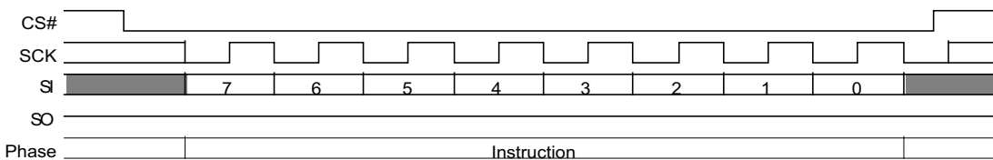
Figure 105. Erase Resume (ERRS 7Ah) Command Sequence
