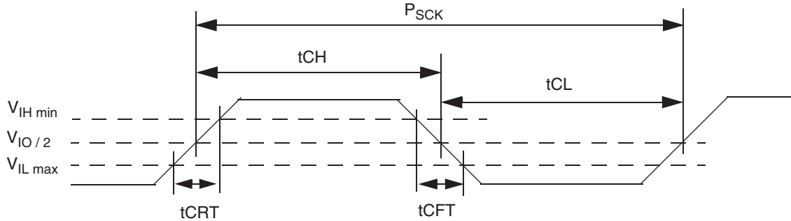
Figure 30. Clock Timing
