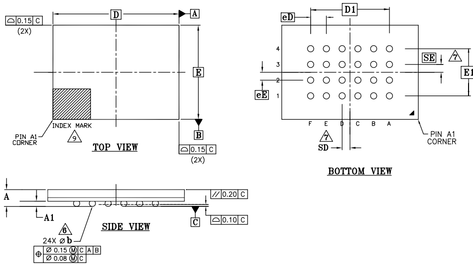
Figure 44. Ball Grid Array 24-Ball 6x8 mm (FAC024)
