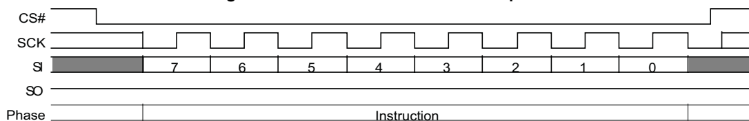
Figure 103. Bulk Erase Command Sequence
