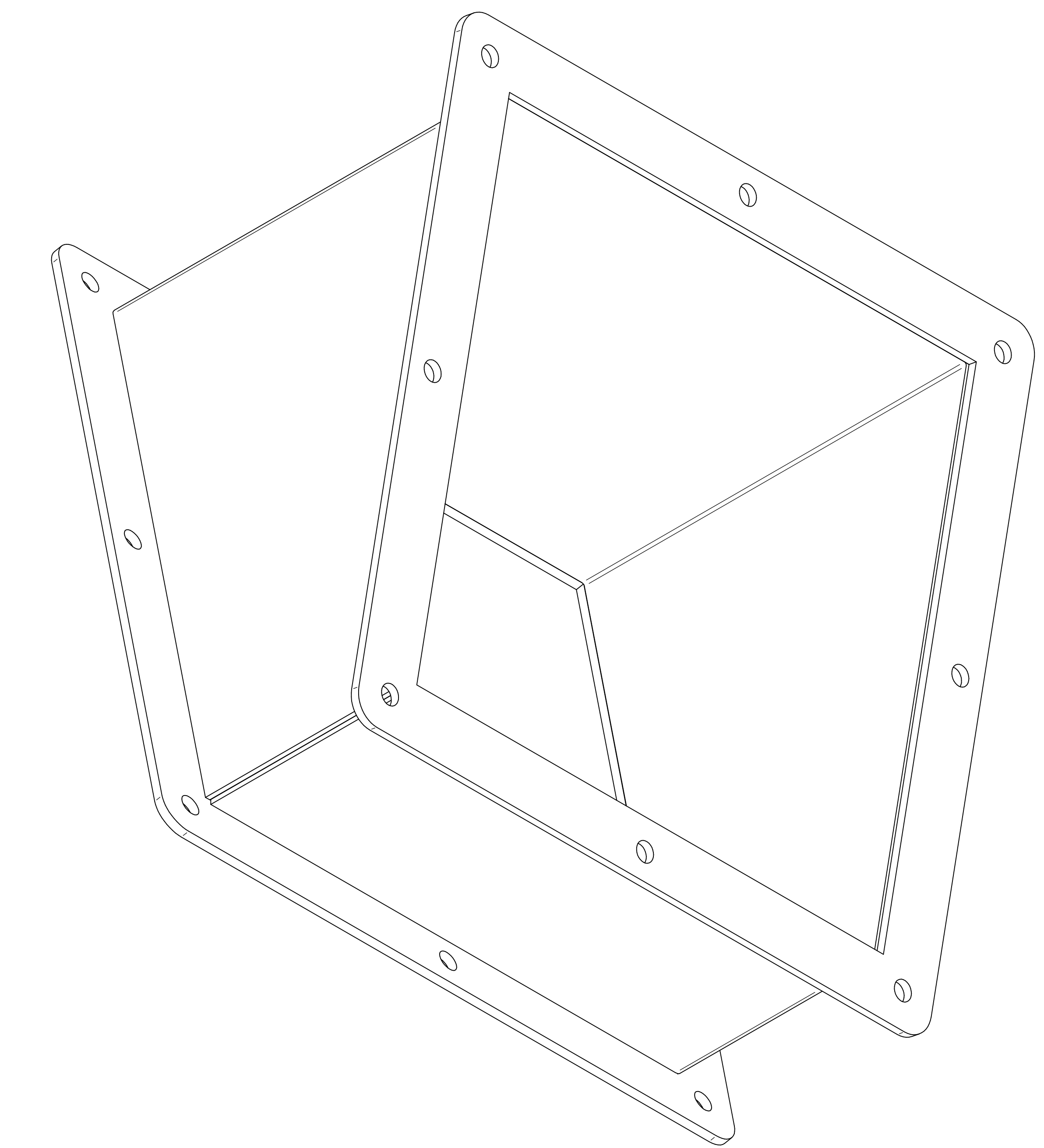
ISOMETRIC VIEWS
