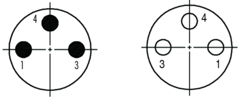
M8 3-PIN MALE M8 3-PIN FEMALE
