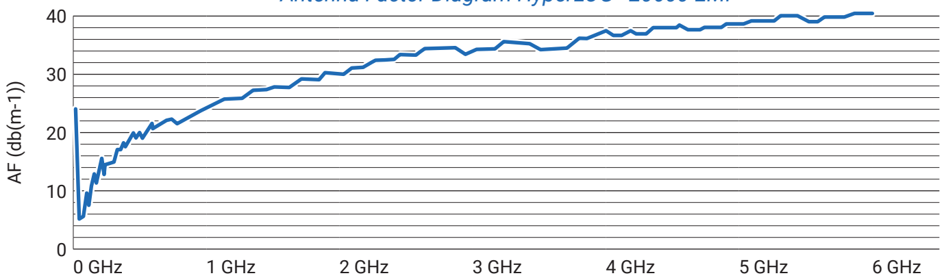
Antenna Factor Diagram HyperLOG® 20600 EMI
