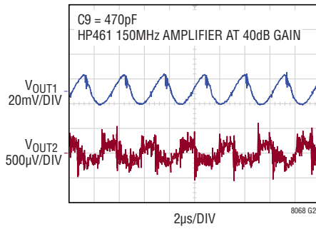
Output Noise and Ripple DC2358A, 200mA Load Current
