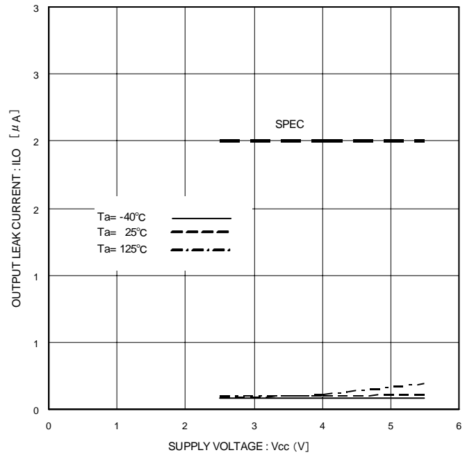
Figure 12. Output Leakage Current ILO(SO)(Vcc=5.5V)
