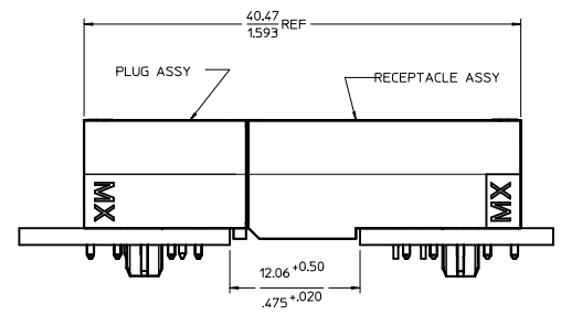
MATED PROFILE (SHOWN MATED TO RIGHT ANGEL RECEPTACLE ASSY)
