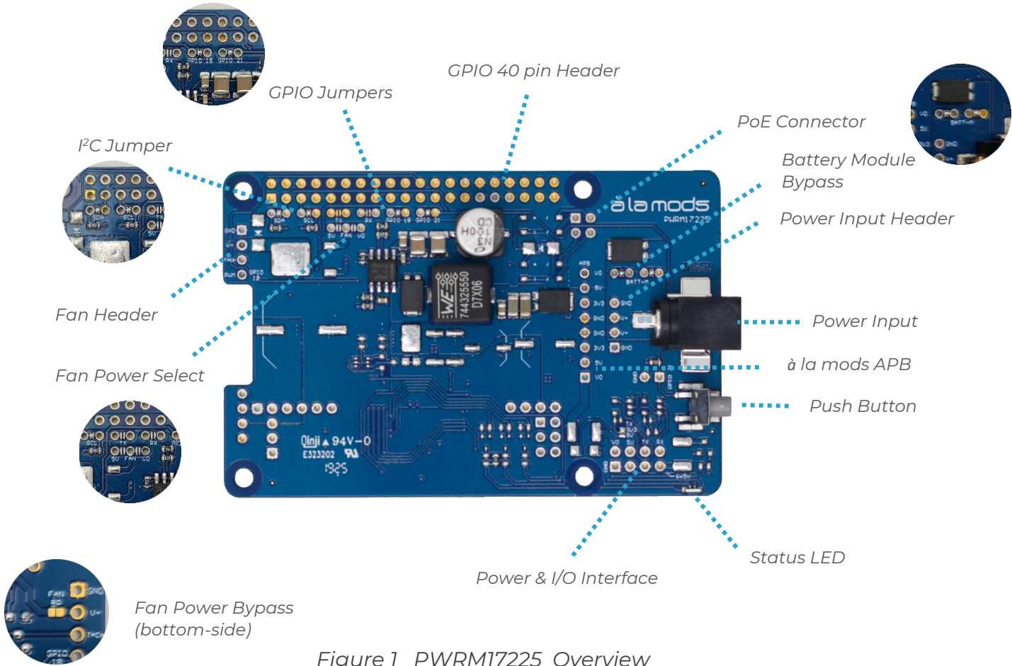
Figure 1 PWRM17225 Overview
