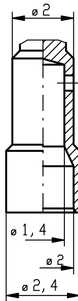
Detail "X" M 10:1
